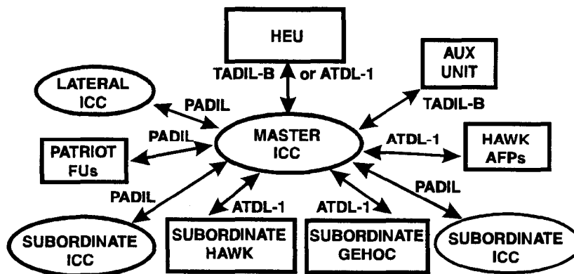
Figure G-13. PDB-3 data link software capability.
