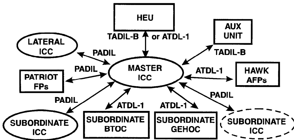
Figure 5-7. Master ICC configuration.
