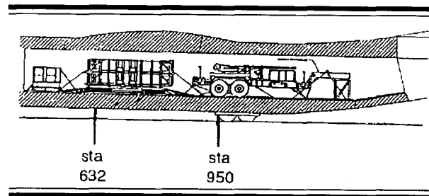
Figure E-4. Launching station, guided missile, C-141.
